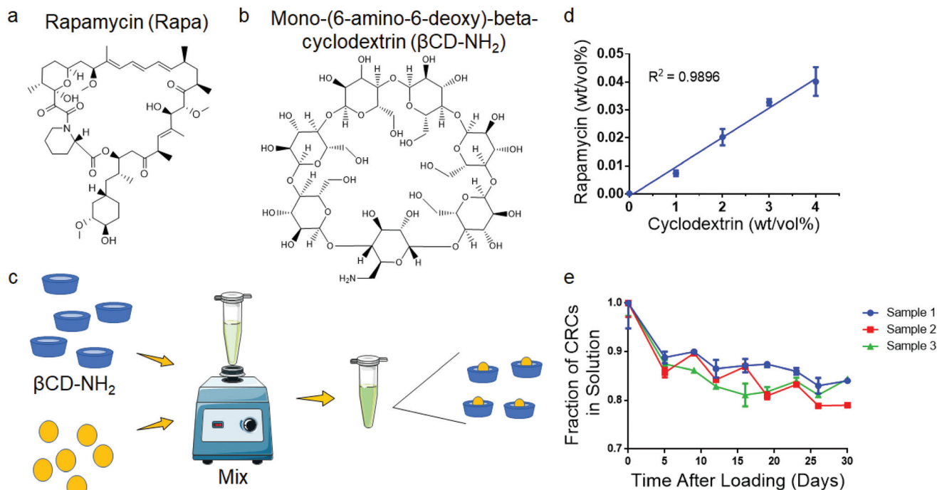
Fig. 1 Complexation with mono-(6-amino-6-deoxy)-beta-cyclodextrin enhances the aqueous solubility of rapamycin. Chemical structure of (a) rapamycin (Rapa) and (b) mono-(6-amino-6-deoxy)-beta-cyclodextrin ( \beta CD-NH 2 ). (c) Schematic for \beta CD-Rapa complexes (CRC). (d) Quantification of the Rapa loading in \beta CD-NH 2 . (e) Stability of CRC in solution over 30 days. Data in (d) represent the mean \pm s.d. for n = 3 independent experiments. Data in e represent the mean \pm s.d. for n = 3 technical replicates.
