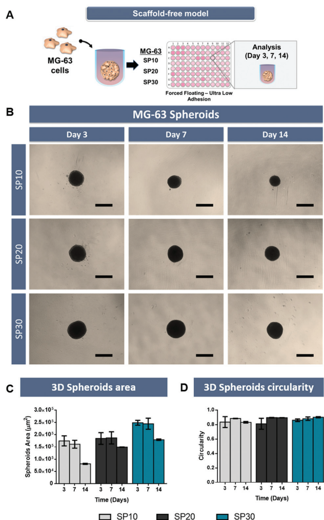
Fig. 1 Optimization of 3D MG-63 spheroids with different cellular densities SP10 – 10 000, SP20 – 20 000 and SP30 – 30 000 cells, and their evolution from 3 to 14 days of culture. (A) Schematics of osteosarcoma spheroids assembly via the liquid overlay technique in ultra-low adhesion (ULA) plates; (B) 3D spheroids morphological analysis by optical contrast microscopy; (C) spheroids area quantification; (D) quantitative circularity measurements (1 = perfect circle, 0 = line). Data is presented as mean \pm s.d., n = 5 . Scale bar = 500 \mu\text{m} .
