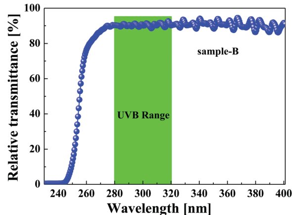
Fig. 2 Relative transmittance through a p-AlGa x N UV-B LED (sample-B).
