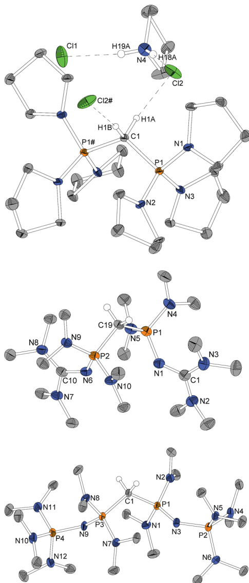
Fig. 2 Molecular structure of 4 · 2HCl with pyrrolidinium chloride as cocrystallite as well as of 1 · 2HBF 4 and 2 · 2HBF 4 (only one of the two independent molecules depicted, structure factors given for both). Peripheral hydrogen atoms and BF 4 − anions omitted for clarity, ellipsoids at 50% probability. # marked atoms generated via a 2-fold axes through C1. Selected bond length/Å and angles/°: 4 · 2HCl P1–C1 1.799(1), P1–N1 1.612(2), P1–N2 1.630(2), P1–N3 1.616(2), P1–C1–P1# 119.5(1), N1–P1–C1 103.26(9), N2–P1–C1 109.07(7), N3–P1–C1 115.21(8), N1–P1–C1–P1# 177.03(7), C1–H1A...Cl2 3.600(2), 173.8; C1–H1B...Cl2# 3.600(2), 173.8; N4–H18A...Cl2 3.048(2), 174(3); N4–H19A...Cl1 3.018(2), 172(3). 1 · 2HBF 4 P1–C19 1.820(2), P1–N4 1.644(2), P1–N5 1.639(2), P1–N1 1.580(2), N1–C1 1.330(3), N2–C1 1.351(3), N3–C1 1.346(3), P2–C19 1.822(2), P2–N9 1.640(2), P2–N10 1.643(2), P2–N6 1.586(2), N6–C10 1.335(3), N7–C10 1.332(3), N8–C10 1.349(3), P1–C19–P2 113.4(1), N4–P1–C19 104.3(1), N5–P1–C19 109.7(1), N1–P1–C19 110.8(1), C1–N1–P1 136.1(2), N9–P2–C19 105.4(1), N10–P2–C19 108.8(1), N6–P2–C19 111.8(1), C10–N6–P2 132.6(2), N4–P1–C19–P2 169.1(1), N9–P2–C19–P1 165.2(1). 2 · 2HBF 4 P1–C1/P5–C22 1.820(4)/1.822(4), P1–N1/P5–N19 1.626(4)/1.630(4), P1–N2/P5–N20 1.642(4)/1.650(4), P1–N3/P5–N21 1.573(4)/1.571(4), P2–N3/P6–N21 1.582(4)/1.589(4), P2–N4/P6–N22 1.648(4)/1.639(4), P2–N5/P6–N23 1.639(4)/1.639(4), P2–N6/P6–N24 1.650(4)/1.655(4), P3–C1/P7–C22 1.819(5)/1.817(5), P3–N7/P7–N13 1.636(4)/1.645(4), P3–N8/P7–N14 1.647(4)/1.635(4), P3–N9/P7–N15 1.575(4)/1.567(4), P4–N9/P8–N15 1.577(4)/
