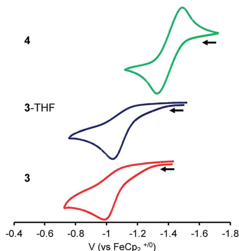
Fig. 3 CVs of 3 , 3-THF and 4 with 0.1 M [ ^m\text{Pr}_4\text{N} ][ \text{BAR}_4^{\text{F}} ] electrolyte in DFB (scan rate of 100 mV \text{s}^{-1} ; collected under Ar).
