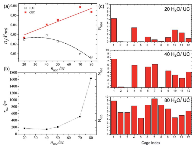
Fig. 24 (a) Self-diffusivities of water (empty symbols and dashed lines) and the center of excess charge (full symbols and solid lines) simulated at 400 K in \text{UiO}-66(\text{Zr})-(\text{CO}_2\text{H})_2 as a function of water loading defined as the number of water molecules ( n_{\text{H}_2\text{O}} ) per unit cell (uc). (b) Residence time of water molecules in the cages of \text{UiO}-66(\text{Zr})-(\text{CO}_2\text{H})_2 averaged over aMS-EVB3 trajectories obtained at 400 K as a function of water loading. (c) Simulated distribution of water in the tetrahedral (from 1 to 8) and octahedral (from 9 to 12) cages of \text{UiO}-66(\text{Zr})-(\text{CO}_2\text{H})_2 at 400 K. Reproduced from ref. 84 with permission from American Chemical Society, Copyright 2017.
