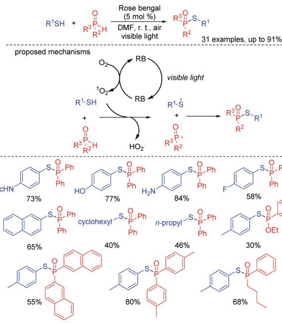
Scheme 24 Construction of S-P(O) bonds.
