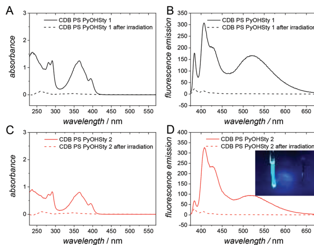
Fig. 4 UV Vis (A and C) and fluorescence spectra (B and D, \lambda_{\text{exc.}} = 344 \text{ nm} ) of CDB PS PyOHSty 1 and 2 before and after exposure to LED irradiation (430–435 nm) showing the presence of pyrene monomers and excimers before light-induced cleavage. The fluorescence of pyrene can also be detected via exposure of the NMR samples to a simple hand-held UV lamp ( \lambda_{\text{exc.}} = 366 \text{ nm} , part D, left: parent polymer, right: after LED light-induced cleavage).
