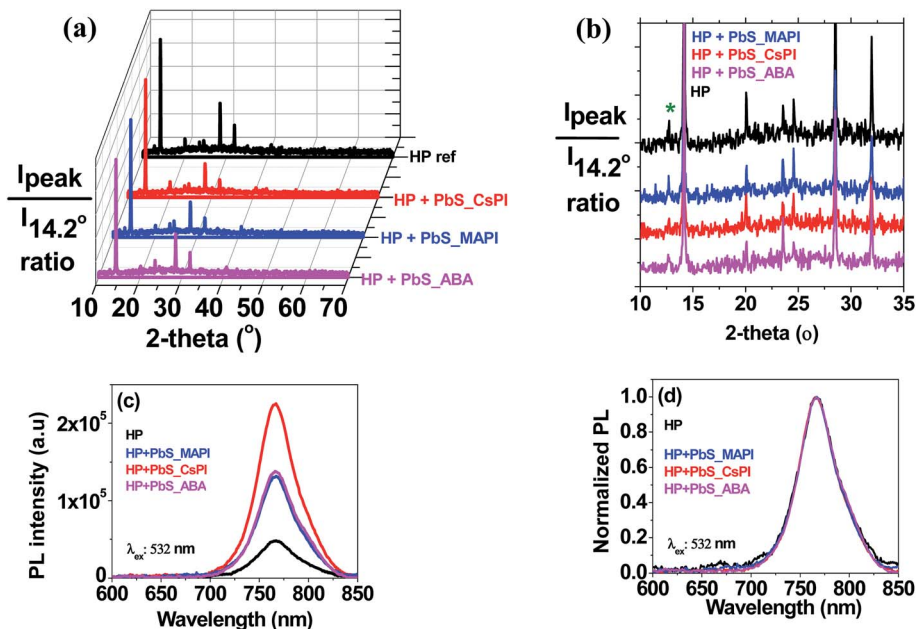
Fig. 2 Crystallographic and optical characterization of perovskite films without (HP) and with PbS QDs ( 50 \mu\text{g ml}^{-1} ) deposited on glass of PbS QDs with the different capping ligands including MAPI, CsPI and 4-aminobenzoic acid (ABA). XRD spectra (a) and a zoom-in from 10 to 35° (b) (the * symbol indicates the \text{PbI}_2 diffraction peak); (c) photoluminescence (PL) and (d) normalized PL spectra.
