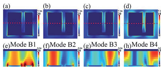
Fig. 4 The electric ( |E| , in the resonator central plane) fields of the frequency points B1 (a), B2 (b), B3 (c), and B4 (d); the magnetic ( |H_y| , perpendicular to the resonator along the red dotted line) fields of the frequency points B1 (e), B2 (f), B3 (g), and B4 (h).
