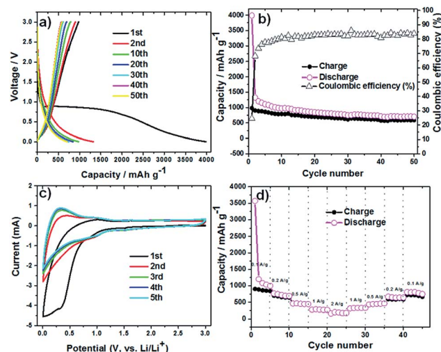
Fig. 3 (a) Charge–discharge curves for \text{Li}_6\text{WO}_6 at a current rate of 100 \text{mA g}^{-1} over the voltage range of 3.0–0.005 V. (b) Capacities versus cycle number of the \text{Li}_6\text{WO}_6 anode over the voltage range of 3.0–0.005 V with a current of 100 \text{mA g}^{-1} . (c) Cyclic voltammetry of the \text{Li}_6\text{WO}_6 electrode at a scan rate of 1 \text{mV s}^{-1} . (d) C-rate testing of the \text{Li}_6\text{WO}_6 anode at different current densities.
