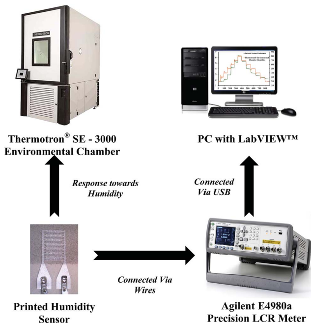
Fig. 7 Experimental setup.
