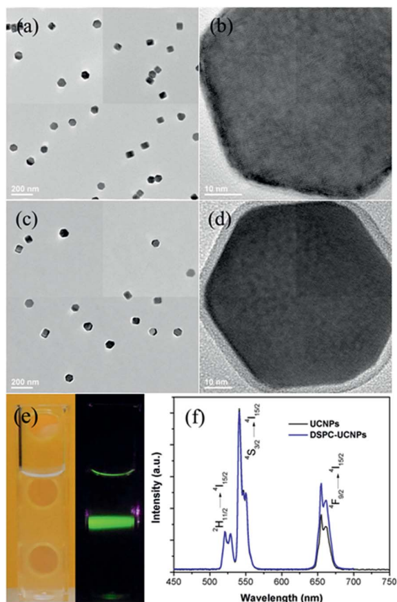
Fig. 4 TEM images of the (a and b) as-prepared and (c and d) phospholipid DSPC coated UCNP s deposited on a TEM grid from a drop of UCNPs cyclohexane solution and DSPC-UCNP water solution, respectively; (e) photographs of the water solution of DSPC-UCNPs without laser illumination and the upconverted visible luminescence under continuous-wave 980 nm laser illumination; (f) room-temperature UCL spectra of the as-prepared UCNP s in cyclohexane and DSPC-UCNP s in water under excitation at 980 nm.
