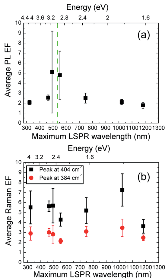
Fig. 4 (a) Average PL peak intensity EF of monolayer \text{MoS}_2 as a function of the LSPR position of Ga NPs. The green line represents the laser wavelength, 532 nm. (b) Average Raman EF of monolayer \text{MoS}_2 peaks at 384 and 404 \text{cm}^{-1} as a function of the LSPR position of Ga NPs. Error bars indicate the standard deviation.
