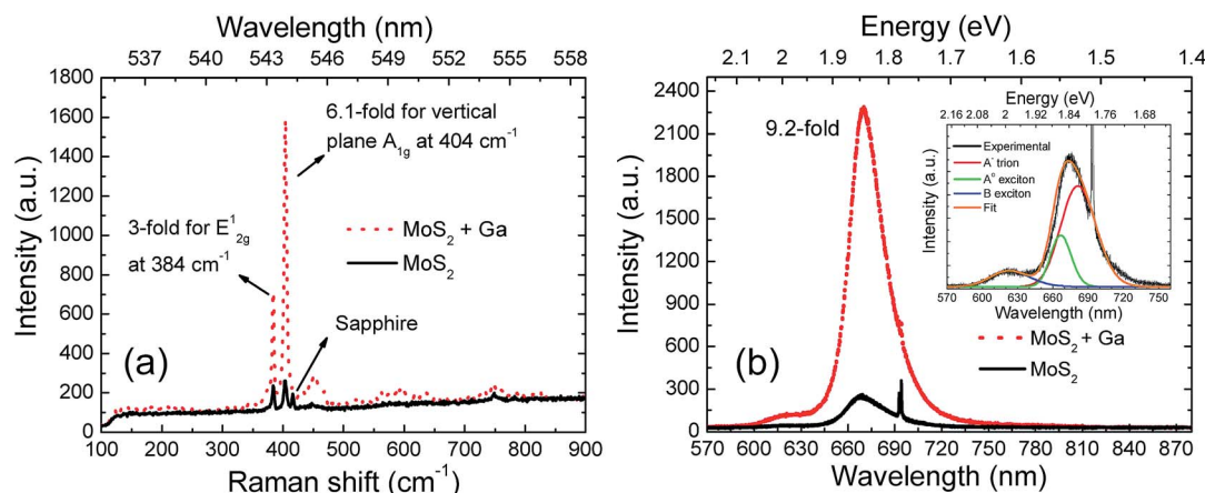
Fig. 3 (a) Raman and (b) PL spectra of a \text{MoS}_2 sample with and without Ga NPs in order to observe the plasmonic enhancement in both cases (excitation at 532 nm). The PL spectra of the pristine \text{MoS}_2 sample is analyzed in the inset of (b) via fitting with a trion and two excitons.
