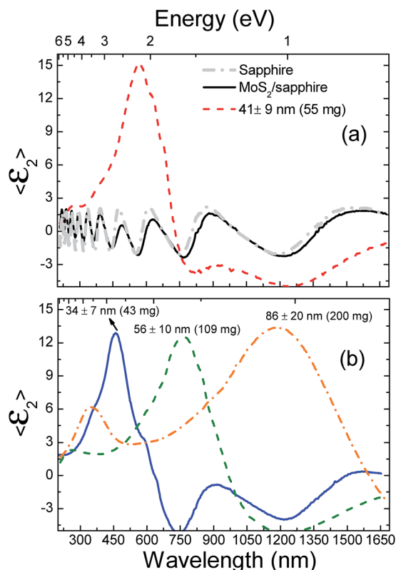
Fig. 2 (a) SE measurement of the sample with Ga NPs of 41 nm radius and reference samples of sapphire and the as-grown \text{MoS}_2/\text{sapphire} . (b) SE measurements of different Ga NPs/ \text{MoS}_2 samples where the LSPR shift with the NP radius can be observed.
