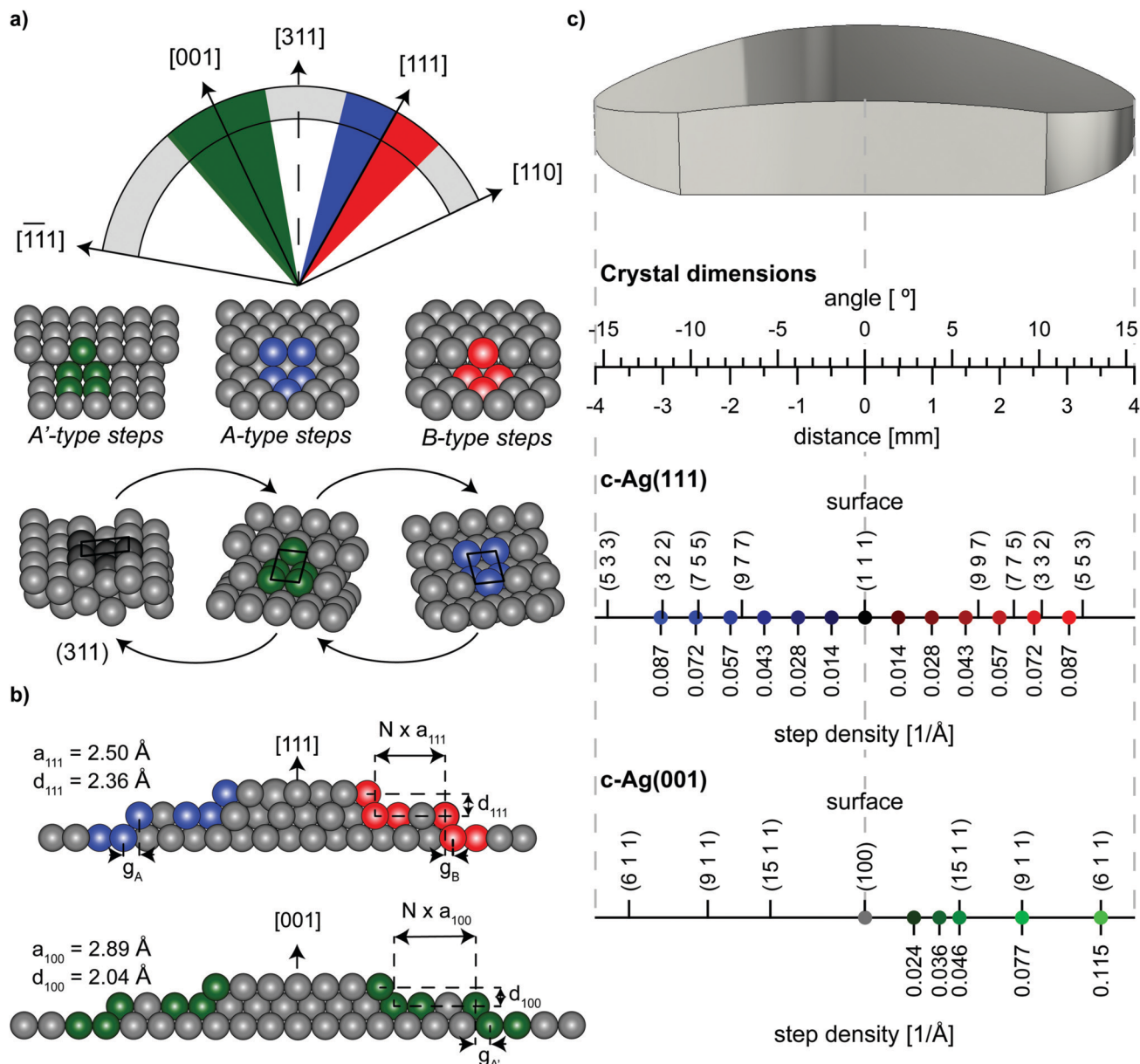
Fig. 1 Schematic drawings of orientation and surface structures of the two curved crystals employed in this study. (a) Orientation of the c\text{-Ag}(001)31^\circ [\bar{1}10] (green) and c\text{-Ag}(111)31^\circ [\bar{1}10] (blue and red) crystals on a cylinder with its rotational axis along [\bar{1}10] . Below the step types that separate (001)/(111) terraces on the two crystals respectively. Also shown, the (311) surface and its unit cell, and how this surface can be seen as consisting of only A- or only A'-type steps. (b) Schematic microscopic side view of the two crystals, indicating parameters used in eqn (1). In the center, the crystals feature wide terraces. As the crystal curves to the sides, steps are introduced to accommodate the macroscopic curvature. (c) Drawing of the macroscopic shape of the crystals linking macroscopic properties of the crystal (angle of curvature, distance from apex), to microscopic properties found on the surface, i.e. Miller indices of surface structures at specific points of the crystal. Positions of measurements in Fig. 4 are indicated in blue, red, and green with their respective step densities. Step densities for monoatomic steps do not follow the same scale on the two crystals because of different step heights on (001) and (111) terraces, as indicated in (b).
