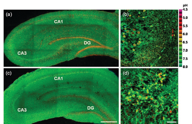
Fig. 43 Pseudocolored ratiometric TPM images ( I_{\text{green}}/I_{\text{IR}} ) of a rat hippocampal slice stained with 30 \mu\text{M} (a and b) 28 and (c and d) 27a . (a and c) 120 TPM images along the z-direction at depths of approximately 90–180 \mu\text{m} were accumulated to visualize the overall pH distribution with 10 \times magnification. (b and d) Higher magnification images (63 \times ) in the regions of DG. Excitation wavelength is 740 nm. Scale bars are (a and c) 300 \mu\text{m} and (b and d) 47 \mu\text{m} . Copyright 2013 American Chemical Society.
