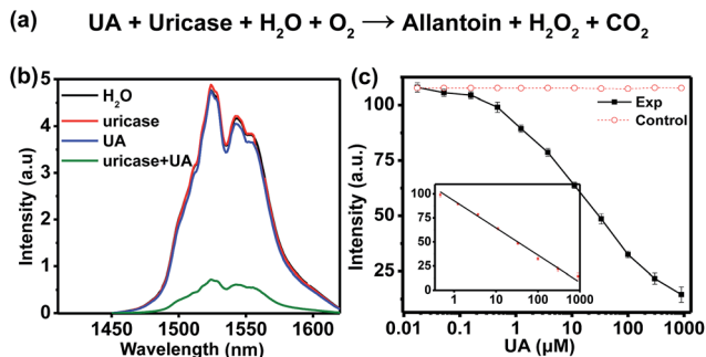
Fig. 4 (a) Chemical equation for the generation of \text{H}_2\text{O}_2 through UA/uricase reaction. (b) NIR-II emission spectra of \text{NaCeF}_4\text{:Er/Yb} NCs ( 0.5 \text{ mg mL}^{-1} ) after the addition of 100 \mu\text{L} of \text{H}_2\text{O} , uricase ( 0.011 \text{ U mL}^{-1} ), UA ( 900 \mu\text{M} ) and uricase ( 0.011 \text{ U mL}^{-1} ) + UA ( 900 \mu\text{M} ), respectively, upon excitation at 980 \text{ nm} . (c) Calibration curve for the UA assay. The control experiment was carried out by replacing UA with \text{H}_2\text{O} under otherwise identical conditions. The inset shows the linear range ( 0.411\text{--}900 \mu\text{M} ) of the calibration curve.
