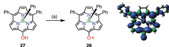
Fig. 10 Synthesis of the subporphyrin meso -oxy radical 28 (isovalue = 0.001). (a) 800 equiv. \text{PbO}_2 , \text{CH}_2\text{Cl}_2 , rt, quant.
