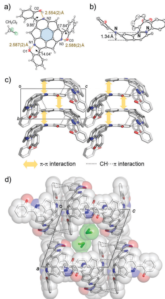
Fig. 2 Crystal structure of (A)-(+)-1. (a) ORTEP model of (A)-(+)-1. The brown dotted lines show the intramolecular hydrogen bonds. (b) The deepest position of the bowl depth. In (a and b), the ellipsoids are shown in 50% probability. (c) Stacking structure viewed from the b axis with intermolecular \pi - \pi (yellow solid arrow) and CH... \pi (grey dotted line) interactions. (d) One-dimensional channel structure with intercolumnar CH... \pi interactions. Green molecules correspond to the encapsulated CH 2 Cl 2 . The colour codes in each of the images in this figure are: C, grey; N, blue; O, red; Cl, light green; however, (e) in (a), the hydrogen atoms are omitted for clarity.
