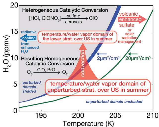
Fig. 8 An example of the three-dimensional dependence of heterogeneous catalytic conversion of inorganic chlorine ( \text{Cl}_2 \approx \text{HCl} + \text{ClONO}_2 ) on temperature, water vapor and sulfate loading is displayed in a manner that distinguishes rapid conversion of Cl 2 to free radical form in the shaded region (with the threshold defined as 10% chlorine activation in the first diurnal period) from the unshaded region for which there is virtually no Cl 2 to ClO conversion. This establishes the photochemical framework for the analysis of convective addition of water, sulfate addition by volcanic injection or overt sulfate addition for solar radiation management (SRM), or combinations thereof. The broad blue line dividing the perturbed and unperturbed domains corresponds to a sulfate reactive surface area of 2 \mu\text{m}^2 \text{cm}^{-3} ; the green line represents a shift in sulfate reactive surface area to 20 \mu\text{m}^2 \text{cm}^{-3} .
