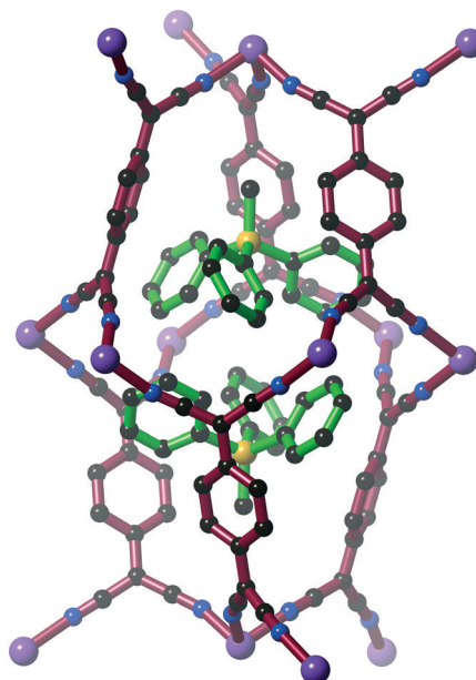
Fig. 12 The structure of (\text{MePPh}_3)_2[\text{M}_{12}(\text{TCNQ})_3] ( \text{M}^{\text{II}} = \text{Zn, Ni, Co, Fe} ) (65–68) in which there is a significant twist in the TCNQ ^{2-} ligands. Pairs of \text{MePPh}_3^+ cations (green) occupy the intra-framework cavities.
