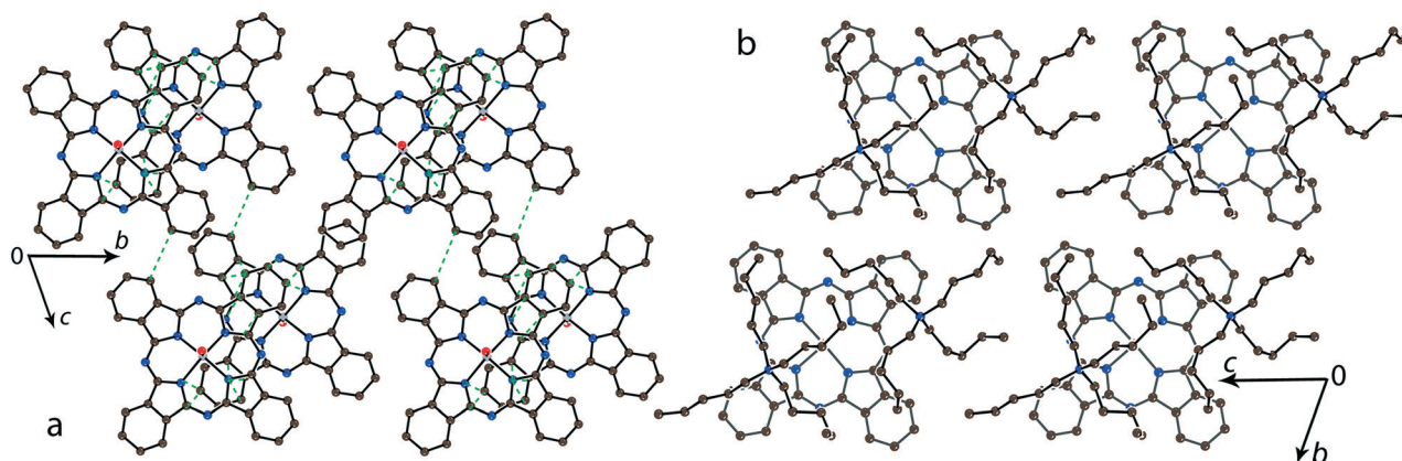
Fig. 4 (a) View of the phthalocyanine layer composed of the \pi -stacking [\{\text{Ti}^{\text{IV}}\text{O}(\text{Pc}^{3-})\}^-]_2 dimers in 4 . Short van der Waals C...C,N contacts are shown by green dashed lines. (b) Projection of the \text{Pent}_4\text{N}^+ layer on the phthalocyanine layer. Only one phthalocyanine from the dimer is shown (bonds are shown in grey).
