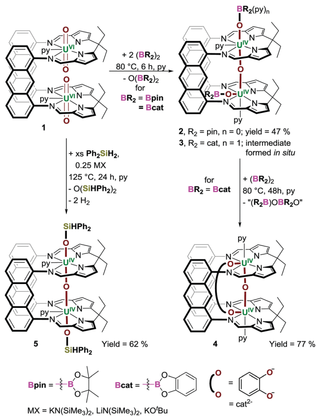
Scheme 1 Diborane or silane-mediated deoxygenation of co-axial uranyl dications to form the new tetracoordination [OUOUO] 4+ 2 , 3 , and 5 , with either trans -, cis - (for boron) or trans -, trans - (for silicon) geometry, and the further deoxygenation of 3 to afford the UOU-containing 4 .
