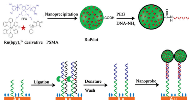
Fig. 16 Schematic diagrams of (A) Preparation of RuPdots nanoprobe using PFO, hydrophobic \text{Ru}(\text{bpy})_3^{2+} derivative, and PSMA; (B) SNP detection with ligase detection reaction and nanoprobe. (Reprinted with permission from ref. 78. Copyright 2017 American Chemical Society.)
