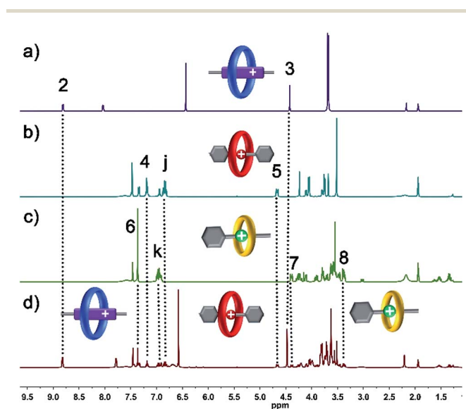
Fig. 1 Partial 1 H NMR spectra (400 MHz, 298 K, CD 3 CN) of (a) 1 : 1 mixture of BPP34C10 ⊃ BPY 2+ , (b) 1 : 1 mixture of DB24C8 ⊃ DBA, (c) 1 : 1 mixture of B21C7 ⊃ BAA and (d) equal molar mixture of BPP34C10, DB24C8, B21C7, BPY 2+ , DBA and BAA.
