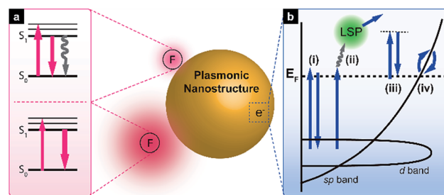
Fig. 1 Schematic illustration of controlling and enhancing PL with plasmonic nanostructures. (a) Jablonski diagram illustrating fluorescence signal changes when emitters are close to or at a short distance from plasmonic nanoparticles. (b) Simplified band diagram of gold showing a possible electronic transition for direct PL.
