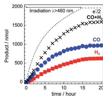
Fig. 4 Time courses of the chemical products ( \text{CO} and \text{H}_2 ) and a half amount of electrons passing through the RuRe / CuGaO 2 photocathode under continuous visible-light irradiation ( \lambda_{\text{ex}} > 460 nm) at -0.3 V vs. Ag/AgCl . A 50 mM aqueous solution of \text{NaHCO}_3 (pH 6.6) that was saturated with \text{CO}_2 was used as the electrolyte.
