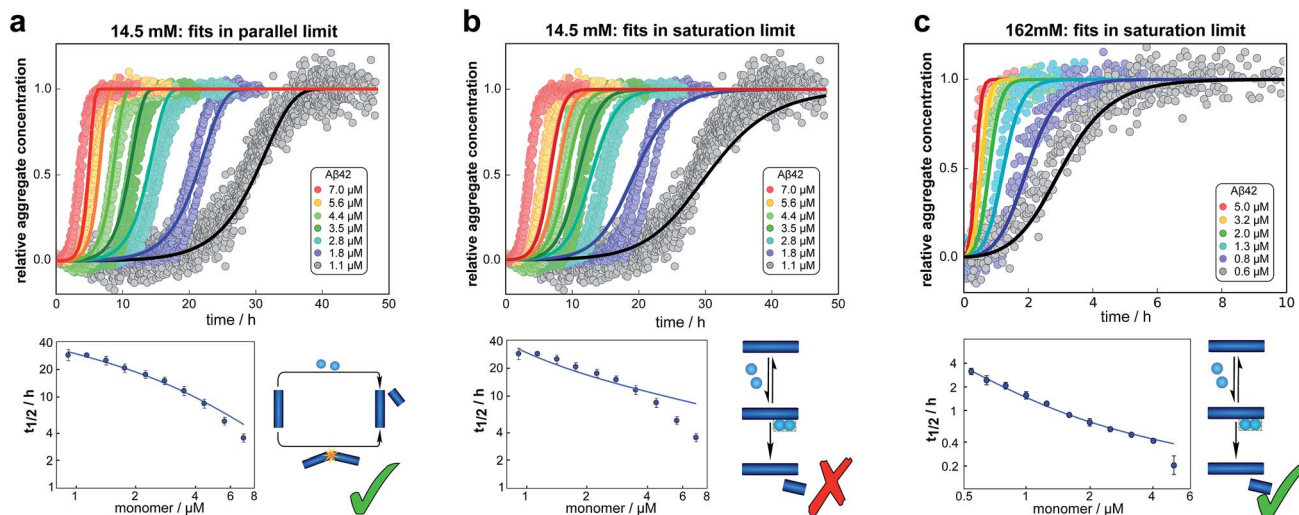
Fig. 4 Global fits of the aggregation curves. (a) The top panel shows a global fit of the parallel limit, eqn (1), with three free parameters, to the all kinetic traces at 14.5 mM ionic strength. Shown below is a fit of just the half time behaviour for the same dataset. (b) The same data set as in (a) is fitted by the saturation limit, eqn (3). The fit of the network in the parallel limit (a) is significantly better than that of the saturation limit (b), the mean squared error in the parallel limit being half of that in the saturation limit. Note in particular how in the saturation limit we fail to reproduce the correct half times, as this limit cannot produce a decrease in scaling exponent with increasing monomer concentration. The saturation mechanism hence cannot explain the data at low ionic strengths. (c) By contrast to (b), a fit of the network in the saturation limit, eqn (3) with three free fitting parameters, to the data at 162 mM ionic strength shows good agreement with the experimental data. For clarity not all sampled concentrations are displayed in the plots of the full time-courses; the fits were, however, performed on the entire dataset (see the ESI, Sections 1.1 and 1.2,† for plots of the full dataset and an explanation of the deviation of the parallel limit fits at high monomer concentrations).
