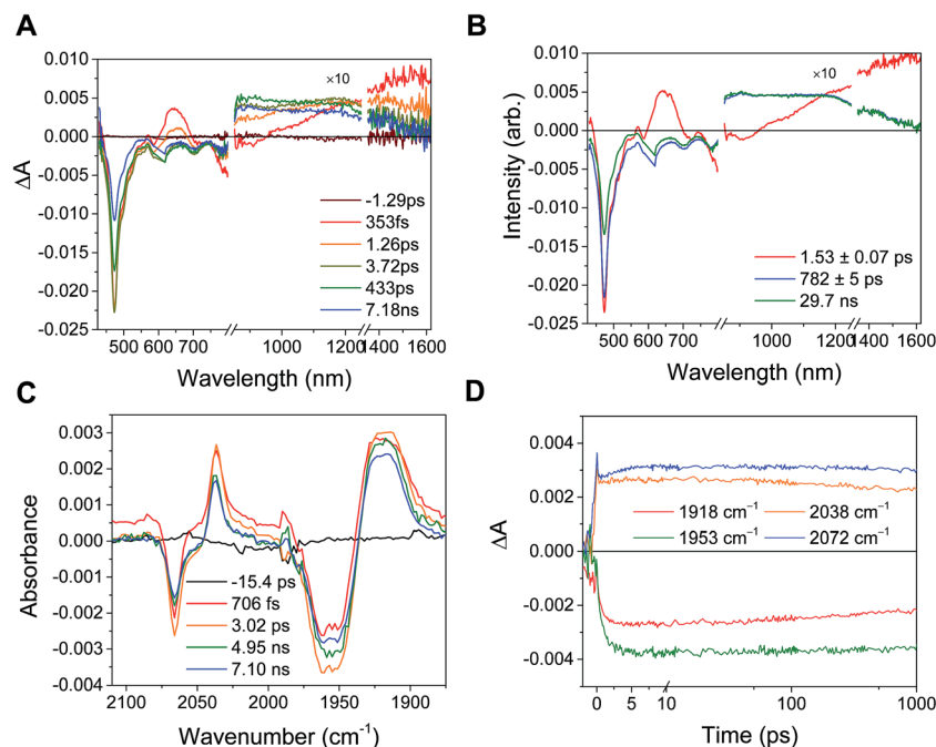
Fig. 10 (A) Transient absorption and (B) species-associated spectra for complex \text{Phbpy-Re-PyPhNDI}^{1-} ( \lambda_{\text{ex}} = 605 \text{ nm} ) showing biphasic back electron transfer kinetics. Kinetic traces and fits are shown in Fig. S7.† (C) fsIR spectra and (D) kinetic traces with fits for complex \text{Phbpy-Re-PyPhNDI}^{1-} ( \lambda_{\text{ex}} = 605 \text{ nm} ) showing monophasic back electron transfer kinetics. The instrument response is approximately 2 ps.
