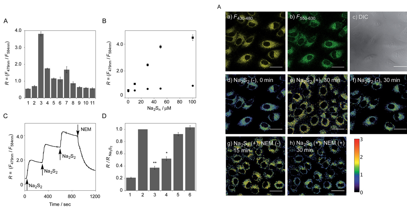
Fig. 3 (A) The ratio value ( R = F_{479\text{ nm}}/F_{584\text{ nm}} ) of 6 in the presence of various thiol species: (1) none, (2) \text{Na}_2\text{S} (50 \mu\text{M} ), (3) \text{Na}_2\text{S}_2 (50 \mu\text{M} ), (4) \text{Na}_2\text{S}_4 (50 \mu\text{M} ), (5) CysSSH (NOC7 (50 \mu\text{M} ) + \text{Na}_2\text{S} (50 \mu\text{M} ) + L-Cys (50 \mu\text{M} )), (6) GSSH (NOC7 (50 \mu\text{M} ) + \text{Na}_2\text{S} (50 \mu\text{M} ) + GSH (50 \mu\text{M} )), (7) mixture of \text{NaOCl} (50 \mu\text{M} ) and \text{Na}_2\text{S} (50 \mu\text{M} ) in 0.1 M \text{NaOH} , (8) mixture of \text{NaOCl} (50 \mu\text{M} ) and \text{Na}_2\text{S} (50 \mu\text{M} ) in 50 mM HEPES buffer (pH 7.4), (9) GSH (5 mM), (10) L-Cys (1 mM), (11) cystine (0.5 mM). Measurement conditions: [\mathbf{6}] = 5 \mu\text{M} in 50 mM HEPES, 10 mM \text{NaCl} , 1 mM \text{MgSO}_4 , 0.4% Tween, pH 7.4, 25 °C. \lambda_{\text{ex}} = 410 \text{ nm} . n = 3 . (B) Change in the fluorescence intensity ratio of 6 (5 \mu\text{M} ) upon addition of \text{Na}_2\text{S}_2 (0–100 \mu\text{M} , ■) and \text{Na}_2\text{S} (0–100 \mu\text{M} , ●). n = 3 . (C) Time-trace plot of the ratio value ( R = F_{479\text{ nm}}/F_{584\text{ nm}} ) of 6 (5 \mu\text{M} ) upon addition of \text{Na}_2\text{S}_2 (30 \mu\text{M} at 30, 300, and 600 s) and N -ethylmaleimide (NEM, 500 \mu\text{M} at 900 s), n = 3 . (D) The reverse change of the ratio value ( R = F_{479\text{ nm}}/F_{584\text{ nm}} ) of 6 induced by the reactive species. Each bar represents R value of: (1) 6 (5 \mu\text{M} ), (2) the hydropersulfide adduct of 6 (5 \mu\text{M} ) with \text{Na}_2\text{S}_2 (50 \mu\text{M} ), (3) the adduct + \text{NaOCl} (100 \mu\text{M} ), (4) the adduct + NEM (200 \mu\text{M} ), (5) the adduct + GSH (5 mM), and (6) the adduct + L-Cys (1 mM). Measurement conditions: 50 mM HEPES, 10 mM \text{NaCl} , 1 mM \text{MgSO}_4 , 0.4% Tween, pH 7.4, 25 °C. \lambda_{\text{ex}} = 410 \text{ nm} . n = 3 ; * P < 0.05 , ** P < 0.01 vs. hydropersulfide adduct of 6 with \text{Na}_2\text{S}_2 (lane 2).
