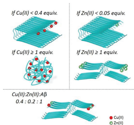
Fig. 2 This figure resumes the aggregation with different Cu(II) : Zn(II) : Aβ ratios. 60 Zn is the ion that dominates the Aβ metal-induced assembly even in the presence of Cu. For all of these aggregation experiments, metal ions have been added at the beginning, i.e. these are metal-induced aggregations.
