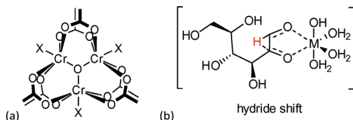
Fig. 13 (a) MIL-101Cr SBU, X = F, OH or solvent; (b) homogeneous metal catalyzed hydride shift in glucose-to-fructose isomerization. The figure was redrawn from ref. 111.
