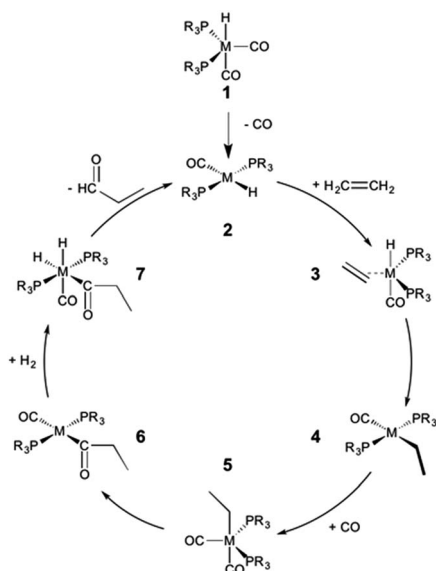
Fig. 2 Mechanism for the Rh-catalysed hydroformylation of an olefin. M = Rh, R = Ph.
