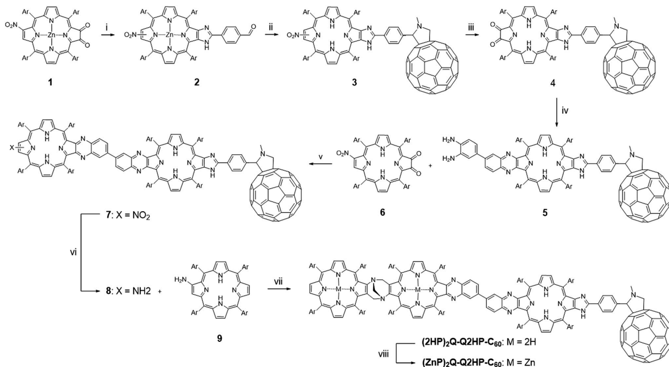
Scheme 1 Reagents and conditions: (i) terephthalaldehyde, \text{NH}_4\text{OAc} , \text{CHCl}_3 , reflux (90%); (ii) 1 , \text{CH}_2\text{Cl}_2 , \text{HCl} , stir (89%); 2 , fullerene, N -methylglycine, toluene, reflux (75%); (iii) 1 , \text{SnCl}_2 \cdot 2\text{H}_2\text{O} , \text{HCl}/\text{Et}_2\text{O} , stir; 2 , \text{CH}_2\text{Cl}_2 , photooxidation (54%); (iv) 3,3' -diaminobenzidine, \text{CH}_2\text{Cl}_2 , stir (80%); (v) \text{CH}_2\text{Cl}_2 , stir (56%); (vi) \text{SnCl}_2 \cdot 2\text{H}_2\text{O} , \text{HCl} , \text{CH}_2\text{Cl}_2 , stir; (vii) THF, \text{HCl}/\text{EtOH} , formaldehyde, stir, 70 °C (16%); (viii) \text{Zn}(\text{OAc})_2 \cdot 2\text{H}_2\text{O} , \text{CH}_2\text{Cl}_2/\text{MeOH} , stir (58%). Ar = 3,5-di- tert -butylphenyl.
