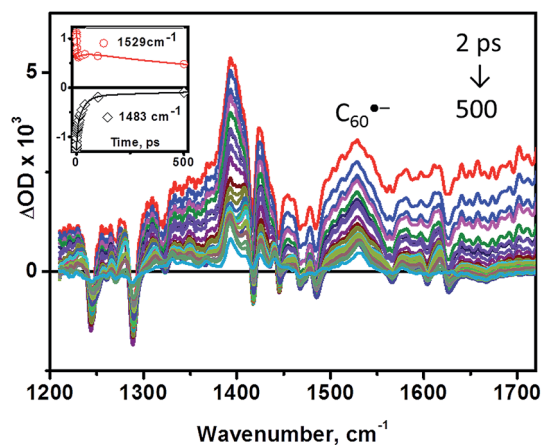
Fig. 4 TRIR spectra of 3 in CD_2Cl_2 solution at 298 K upon laser excitation at 400 nm, ~50 fs pulse, at different time delays. Inset: kinetics at selected frequencies. Symbols are experimental points, and the lines are multiexponential fits to the data using the parameters obtained by a global fit, which yielded lifetimes values of 2.5 ( \pm 0.3 ) ps, 31 ( \pm 0.4 ) ps, and 890 ( \pm 17 ) ps.
