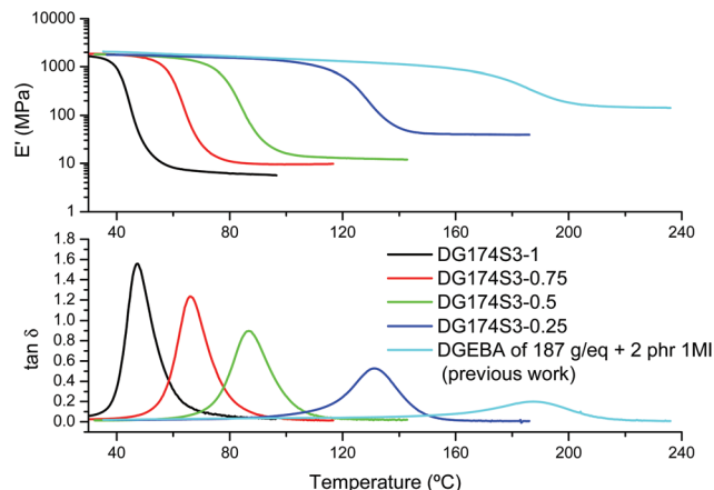
Fig. 6 DMA analysis of DG174S3- r formulations in comparison with a neat epoxy homopolymer formulation from a previous work. 27
