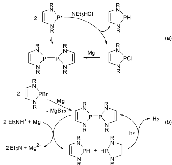
Scheme 14 (a) Reduction of Cl-DAPs to H-DAPs using Mg/Et 3 NHCl via disproportionation of diazaphospholenyl radicals as the key step (R = Dipp, 2-tBuC 6 H 4 ); 15 (b) photocatalytic reductive generation of H 2 (R = Dipp). 61 Both reactions can also be performed with CC-saturated NHPs. Generation of the bis-diazaphospholenyl in (b) can be performed in situ from a Br-NHP precursor.
