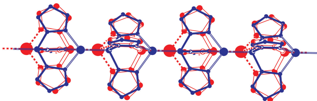
Fig. 8 Disorder in the one-dimensional CuPF coordination chain of [(\text{CH}_3\text{Cu})[\text{PF}_6])_n . Location in the unit cell at (2/3, 1/3, z) , Wyckoff position b . The major disorder component is drawn in red, the minor component in blue. The estimated ratio between the two components is 65 : 35%.
