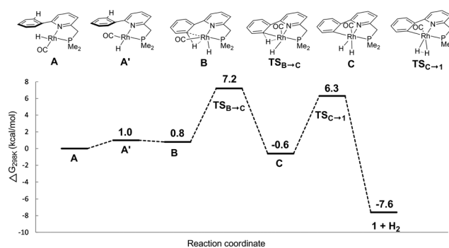
Fig. 3 DFT (BP86, def2-TVZP, disp3) calculated free energy profile ( \Delta G_{298\text{K}}^0 in kcal mol −1 ) of dihydrogen formation from hydride intermediate \text{A}^{\text{Me}} , with methyl instead of tert -butyl groups.
