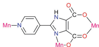
Fig. 13 Section of the structure of [Mn_2(Hpidc)(H_2O) \cdot 2H_2O]_n . 78
