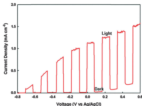
Fig. 36 J–V plot of \text{In}_2\text{S}_3 films obtained from AACVD at 400^\circ\text{C} from [\text{In}(\text{S}_2\text{CN}^1\text{Pr}_2)_3 \cdot 1.5(\text{py})] . Reproduced with permission from ref. 85. Copyright 2013 Royal Society of Chemistry.
