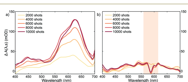
Fig. 3 Change in the absorption spectra of SNO thin crystals measured 28 ms after excitation for different number of 266 nm laser shots ( 1.4 \text{ mJ cm}^{-2} ) a) without using the NOPA photoreversion pulse and b) with the photoreversion pulse ( 2.8 \text{ mJ cm}^{-2} ). The spectral region covered by the NOPA beam is shaded. In this region, the scattered light coming from the NOPA beam reaching the detector produced fluctuations increasing the noise significantly.
