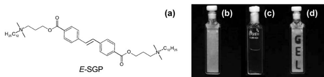
Fig. 8 Molecular structure of alkene-based photoresponsive LMWG. On exposure to UV light, a trans -to- cis isomerisation occurs, leading to a gel-to-sol transition. Reproduced from ref. 39 with permission of the Royal Society of Chemistry.
