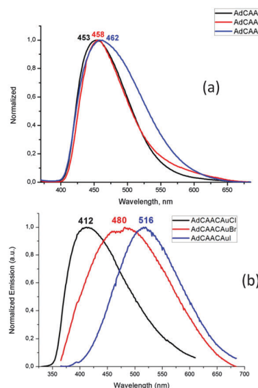
Fig. 2 Emission spectra of (a) (^{\text{Ad}}\text{L})\text{CuX} and (b) (^{\text{Ad}}\text{L})\text{AuX} ( X = \text{Cl}, \text{Br}, \text{I} ) in the solid state (excited at \lambda_{\text{exc}} = 365 \text{ nm} ).
