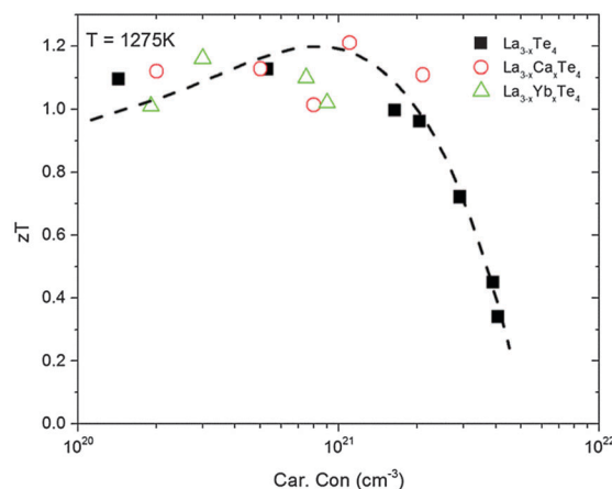
Fig. 12 The thermoelectric figure of merit zT at 1275 K as a function of carrier concentration for La 3−x Ca x Te 4 as compared to La 3−x Te 4 and La 3−x Yb x Te 4 . 7,17 The results fit well to the multi-parabolic band model of La 3−x Te 4 (dashed line).
