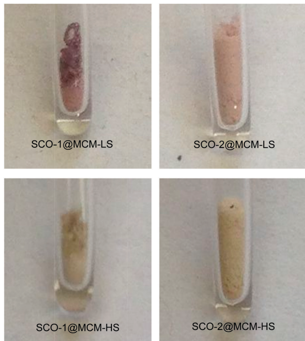
Fig. 1 Photographs showing the color change from LS (room temperature) to HS ( \sim 100\text{ }^{\circ}\text{C} ) for each sample.
