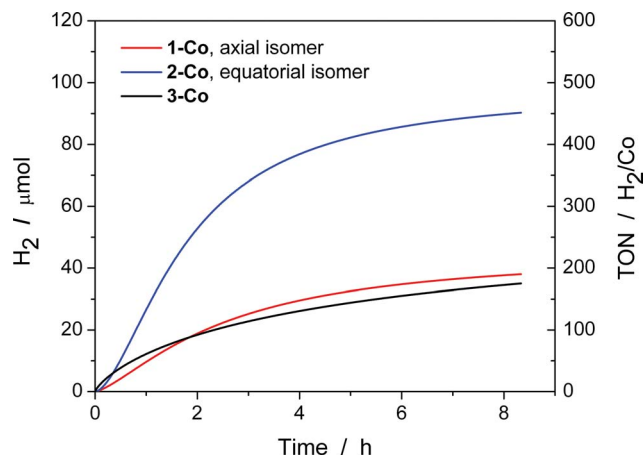
Fig. 8 Photocatalytic H_2 production of 1-Co, 2-Co, and 3-Co with [\text{Ru}(\text{bpy})_3]^{2+} and ascorbic acid under 452 \pm 10 nm (540 mW). H_2 evolution and TON vs. time measured over 8 h of photocatalysis. Conditions: 2.0 \times 10^{-5} M Co(II) catalyst, 3.3 \times 10^{-4} M [\text{Ru}(\text{bpy})_3]^{2+} , and 0.3 M H_2A/HA^- at pH 5.5.
