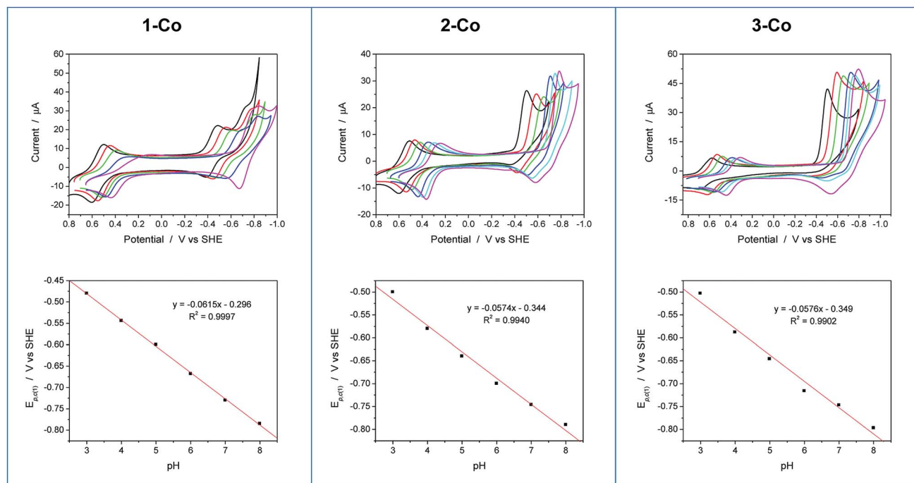
Fig. 5 Cyclic voltammograms as a function of pH and plots of the first reductive peak potential ( E_{p,c(1)} ) vs. pH for 1-Co, 2-Co, and 3-Co. Conditions: 0.9 mM catalyst, 0.03 M buffer, 0.1 M \text{KNO}_3 , 100 \text{ mV s}^{-1} scan rate, glassy carbon electrode (3 mm dia). Note: CV at pH 7 is omitted for clarity in series of CVs for 1-Co. Legend: pH 3 (black), pH 4 (red), pH 5 (green), pH 6 (blue), pH 7 (cyan), pH 8 (magenta).
