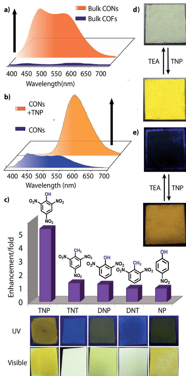
Fig. 6 (a) Photoluminescent spectra of bulk TfpBDH and TfpBDH-CONs ; (b) photoluminescent spectra showing turn on (PL enhancement) of bulk TfpBDH-CONs and with TNP; (c) photoluminescence enhancement plots of different analytes [at 5.4 \times 10^{-5} (M)] with TfpBDH-CONs ; (d and e) solid state sensing (turn on) by TfpBDH-CONs in presence of TNP under visible and UV light (365 nm) which also exhibits the reversible color change from blue to yellow and vice versa upon TEA treatment.
