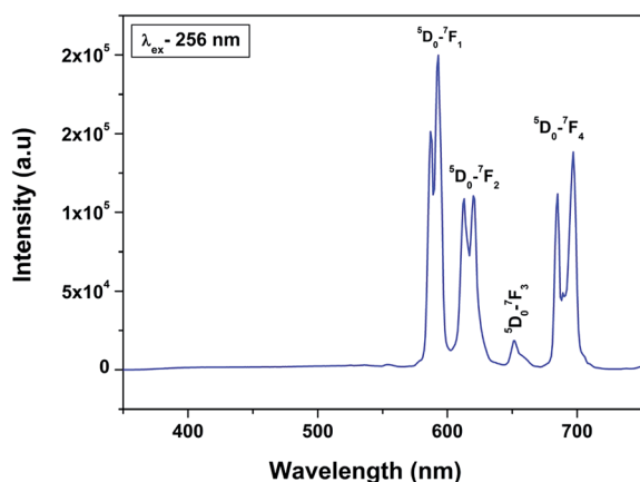
Fig. 6 Emission spectrum of \text{LaPO}_4:\text{Eu}^{3+} (0.5 mol%) at an excitation wavelength of 256 nm.
