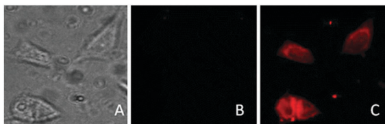
Fig. 68 Top: structure and reaction of RBPH with \text{ONOO}^- ; inset shows the diazo intermediate 69 that forms prior to fragmentation. Bottom: (A) bright-field image of MCF-7 cells incubated with RBPH. (B) Corresponding fluorescence image (C) fluorescence image of MCF-7 cells incubated with RBPH then peroxyntirite. Image reproduced with permission. 282
